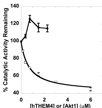
Figure 4. Plots of the % Akt1 kinase activity vs the concentration of hTHEM4 (O) and % hTHEM4 activity vs the concentration of Akt1 (■). The error bars represent the standard deviation of triplicate data points. See SI for details.
