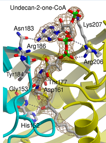
Figure 2. The hTHEM4 active site bound with undecan-2-one-CoA. The mesh defines the initial difference Fourier electron density with the coefficients F_o - F_c and calculated phases prior to adding the ligand to the model. The map is contoured to 2.5 \sigma .
