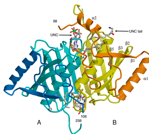
Figure 1. The hTHEM4 dimer with one molecule of undecan-2-one-CoA (UNC) bound to each subunit (A blue and B yellow; N-domain darker shade) and with a third partially disordered molecule of UNC bound to subunit B (UNC tail).
