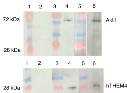
Figure 3. Western blots of the protein fraction eluted from Akt1 antibody-functionalized agarose beads incubated with 150 \mu g of Akt1 and 35 \mu g of hTHEM4-His 6 (Lane 4) or His 6 -hTHEM4 (Lane 6). Lane 2 is the protein from the control in which Akt1 was omitted. Lanes 1, 3, and 5 contain PageRuler Plus Prestained Ladder. The top immunoblot was developed using anti-Akt1 antibody and the bottom using anti-hTHEM4 antibody.
